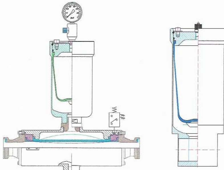
Figure 9. On the left, IN-LINE hygienic dampeners. On the right, BLADDER dampeners with 2 connection ports
