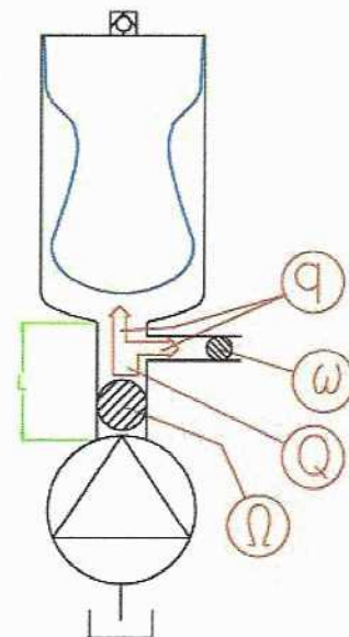
Figure 7. Scheme of the main parameters involved in the in-line assembly of a pulsation damper.
